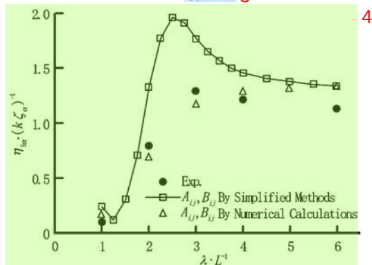
(b) Pitch
