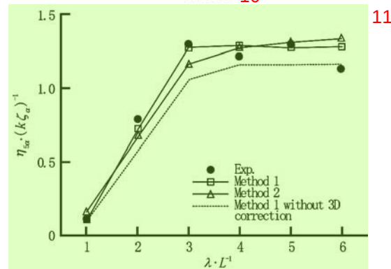
(b) Pitch
