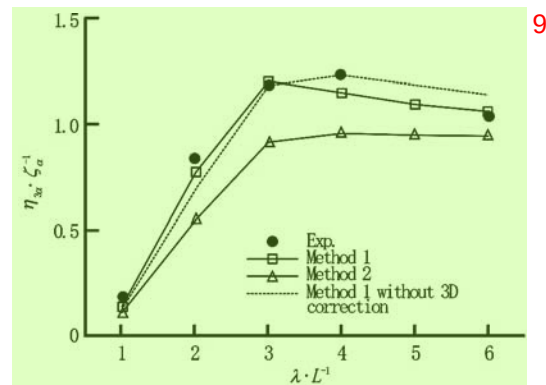
(a) Heave
