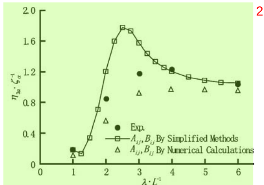
(a) Heave
